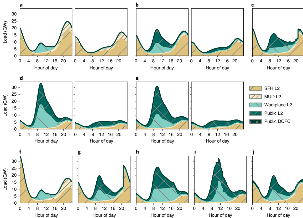
Fig. 2 | Profile of aggregate EV charging demand illustrated for each infrastructure and control scenario. a,b,d,e. The uncontrolled profiles for a typical weekday (left) and weekend (right) are shown for Universal Home access (a); High Home access (b); Low Home, High Work access (d) and Low Home, Low Work access (e). f–j. The weekday profile is shown for one example of each type of control: midnight SFH timers with Universal Home access (f); 9 p.m. SFH timers with High Home access (g); workplace peak minimization with Low Home, High Work access (h); workplace average emissions minimization with Low Home, Low Work access (i); and random SFH timers between 8 p.m. and 2:30 a.m. with High Home access (j) (Methods). Profiles are illustrated for full electrification for the US states in WECC to show the maximum modelled demand. Demand is aggregated in local time for this illustration, but in the simulation the two time zones are reflected and there is a 1 h delay between the timers set on Pacific and Mountain Time. c. Business As Usual is a special case of High Home access with a mixture of residential timers at 8 p.m., 9 p.m., 10 p.m. and midnight and peak minimization workplace control. The weekday and weekend profile for each scenario is repeated to compile the full year's charging demand. L2 stands for Level 2 charging and DCFC stands for Direct Current Fast Charging.
