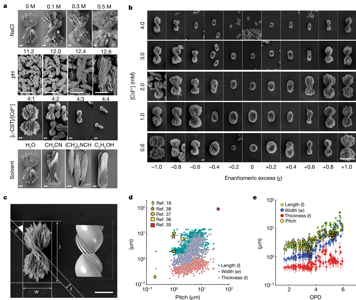
Fig. 3 | Morphological diversity of bowties. a , Effect of NaCl, pH, excess charge (L-CST/Cd), solvent (1:1 water to solvent) on bowtie morphology (water, [Cd^{2+}] = 1\text{ mM} , 4 mM for pH, [L-CST] = 4\text{ mM} ) are shown. Scale bar, 1 \mu\text{m} . b , Continuously variable twist and sizes for bowtie particles obtained for different \chi and [Cd^{2+}] . Scale bar, 5 \mu\text{m} . c , SEM image of a typical bowtie assembly and the corresponding morphological parameters of length ( l ), width ( w ), thickness ( t ) and pitch ( 2w\tan(90 - \theta) ) overlaid. Three-dimensional models
