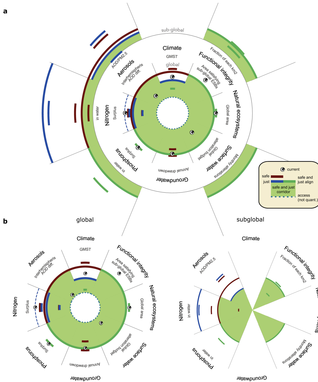
Extended Data Fig. 1 | Alternative visualizations of safe and just Earth system boundaries (Fig. 1). Concentric (a) and parallel (b) visualizations of global (a, inner circle; b, left circle) and sub-global (a, outer circle; b, right circle) safe and just ESBs. Colours are as in Fig. 1. Global rings (a, inner circle;
